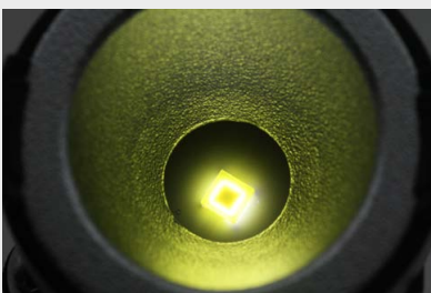
Dimmed white LED with reflector, making use of Shin-Etsu's phosphor blended silicone encapsulant and photo resist coating
