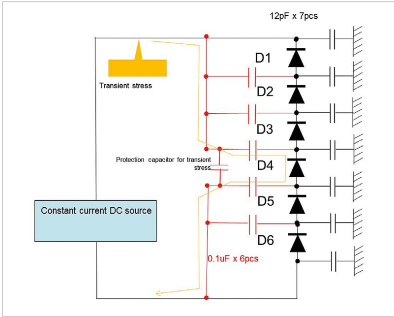
Figure 9: Protection capacitors during normal operation
