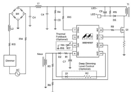
Typical application circuit diagram for a non-isolated phase-cut dimmable single-stage buck-boost LED driver using the 88EM8187
