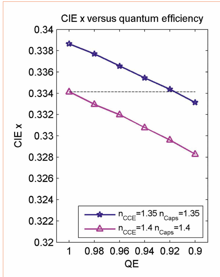
Figure 4: Variation of CIE x values as a function of the quantum efficiency of the phosphor and the refractive index of the silicone for a set-up in accordance with figure 1b for which additionally scattering particles are added to the silicone encapsulation layer
