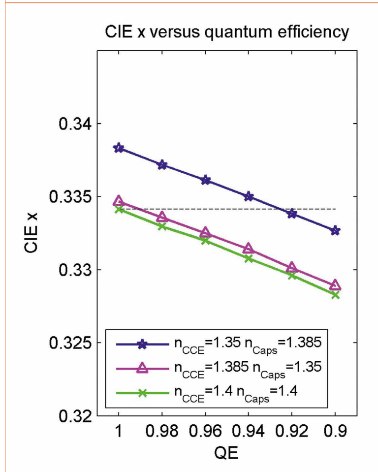
Figure 5: Variation of CIE x values as a function of the quantum efficiency of the phosphor and the refractive index of the silicone for a combination of silicones with different thermo-optic coefficients
