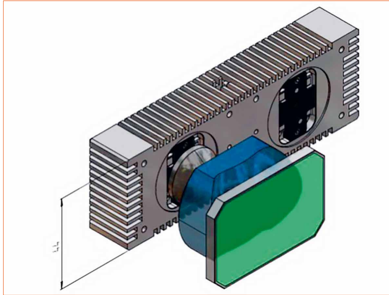
Figure 9: Construction of the low beam demonstrator (only left module shown equipped with optics)
