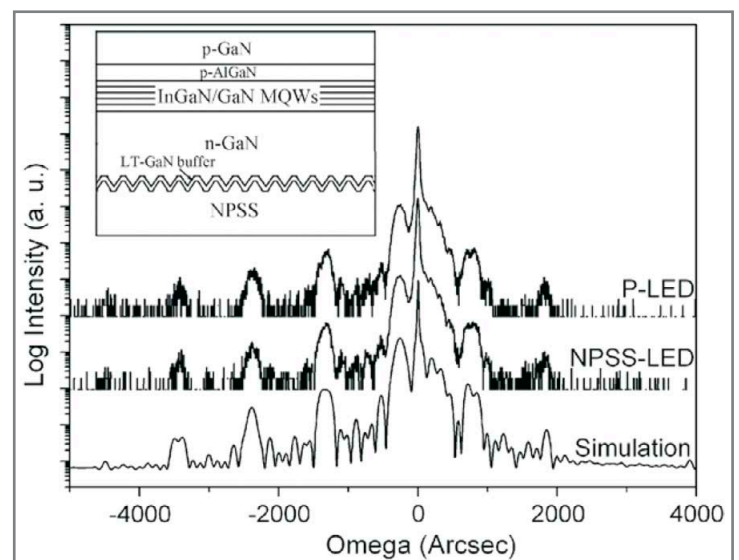
Figure 2: The high resolution triple-axis XRD \omega - 2\theta (0\ 0\ 0\ 2) scans for the P-LED and the NPSS-LED. The lowest curve is the simulation result for the NPSS-LED. The inset is the schematic diagram of the structure of LED epitaxial layers grown on NPSSs
