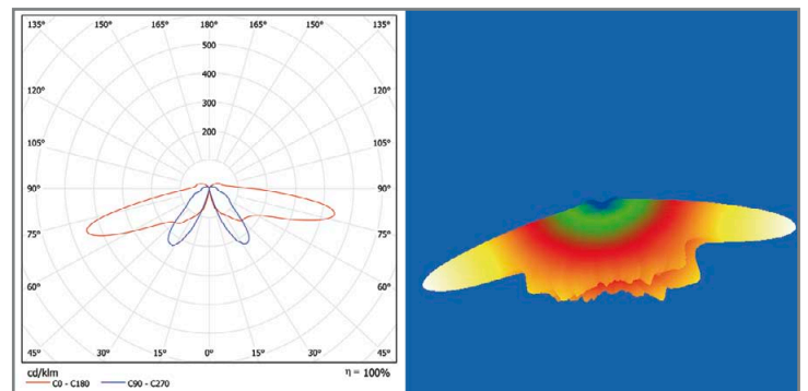
Figure 9: Measurement and simulation results for an existing round shaped reflector
