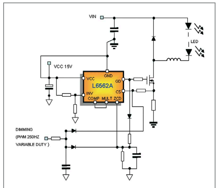
Figure 6: DC/DC LED current control stage
