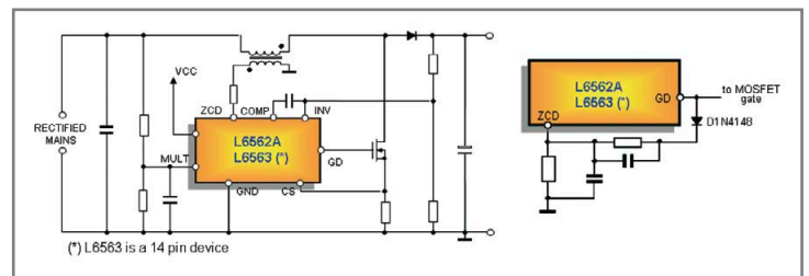
Figure 2: Power factor corrector stage in transition mode (left) and circuitry for fixed-off-time control (right)
