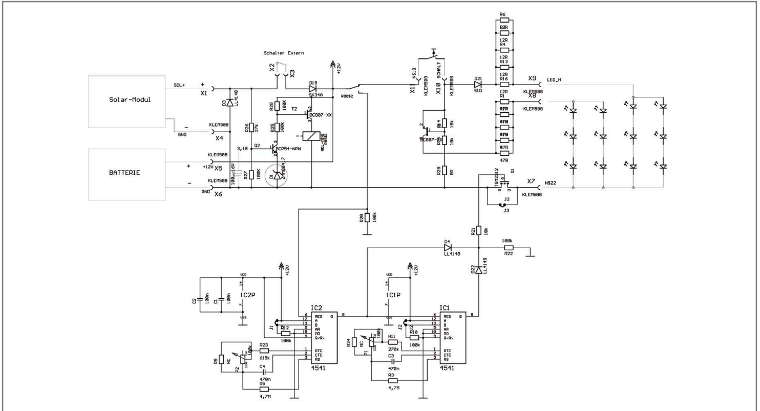
Figure 7: Schematic of the EPS soltec electronics
