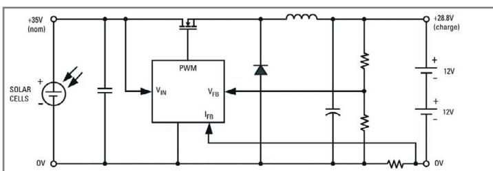
Figure 4: Schematic of Buck regulator battery charger (original)
