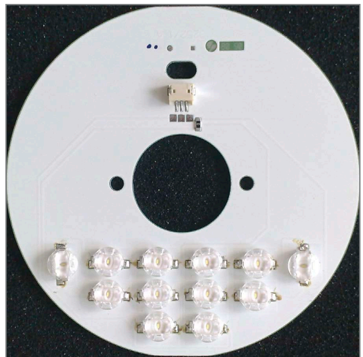
Figure 3: High-performance MCPCB LED board
