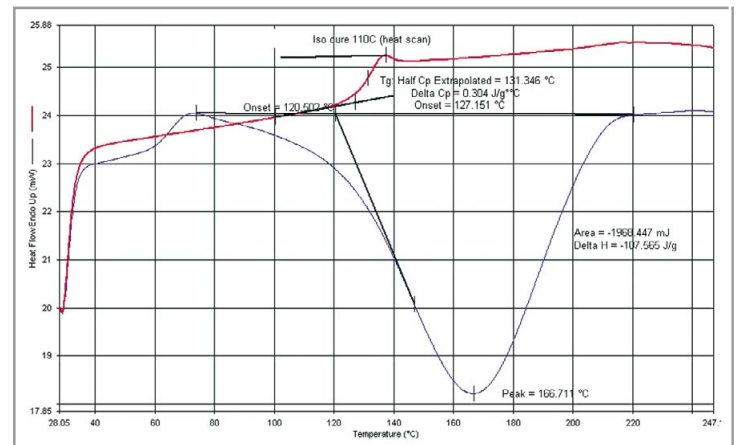
Fig. 1: Isothermal Cure: 110 °C
