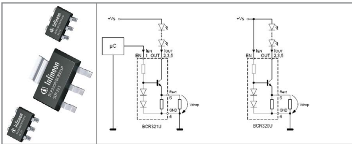
The new BCR320 and BCR420 LED drivers and the typical application circuits: Enabling with PWM by micro controller and enabling by connecting to V_s .
