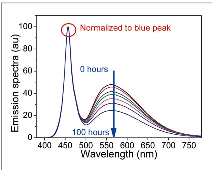
Figure 5: Emission spectra of LEDs submitted to the thermal storage. The spectra have been normalized to the blue peak, in order to underline the lowering of the yellow peak with respect to the blue one.
